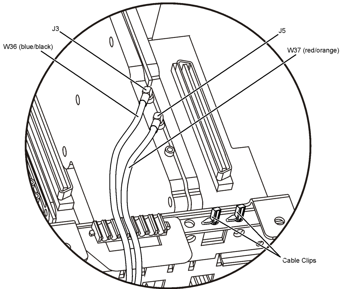
Figure 12 ACPR Cable Connections
