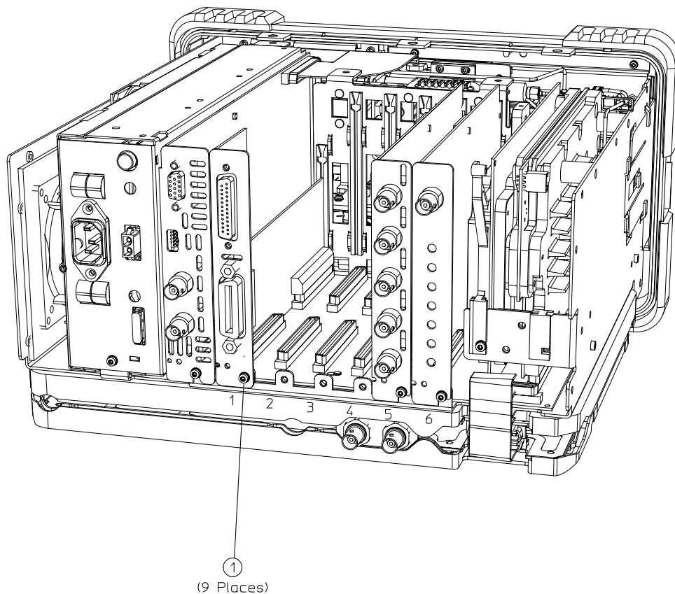
Figure 6 Instrument, Rear View
