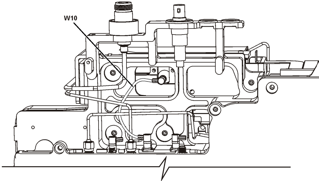
Figure 10 W10 Cable Location
