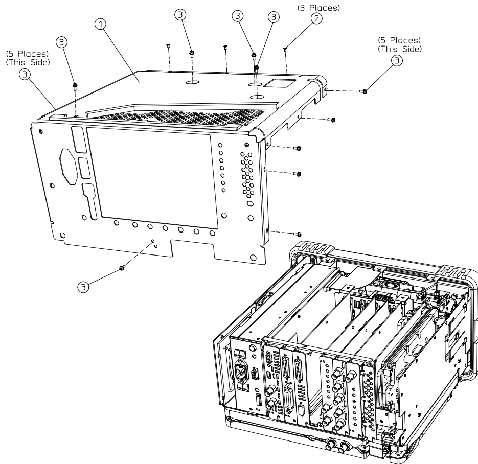
Figure 17 Inner Shield Replacement
