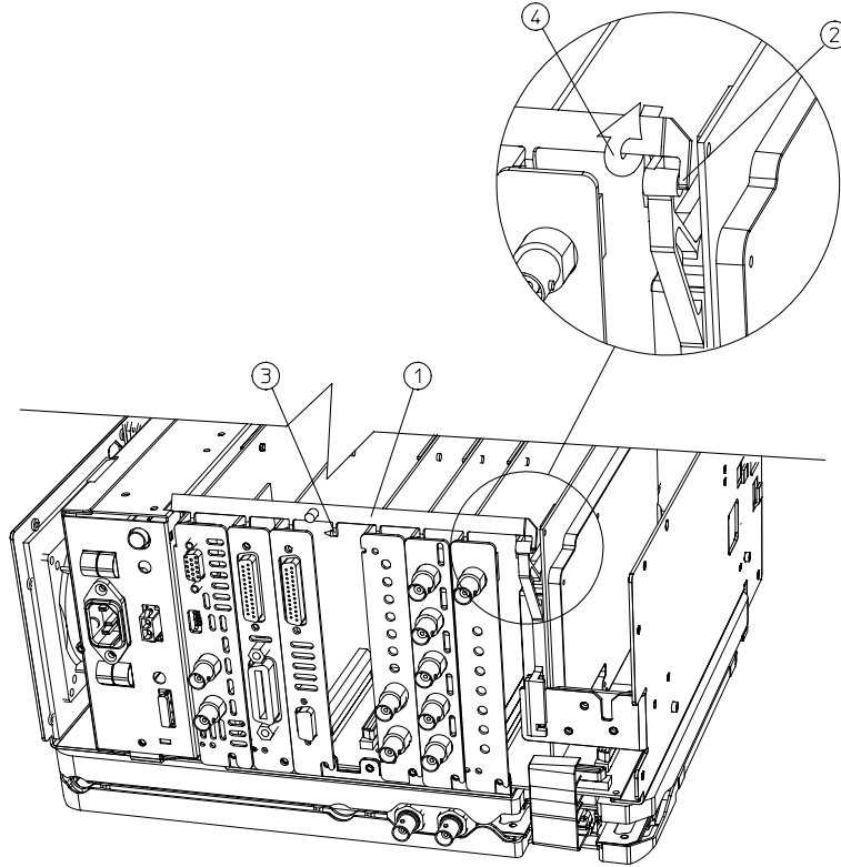
Figure 8 Installing the Vibration Support Bar
