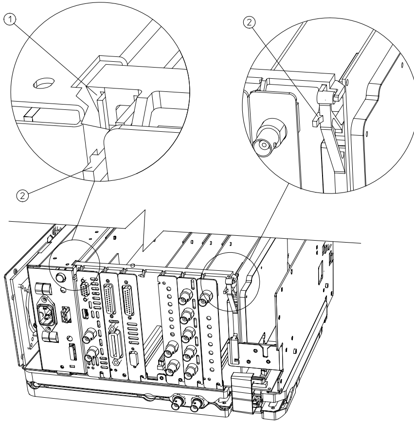
Figure 9 Seating the Vibration Support Bar
