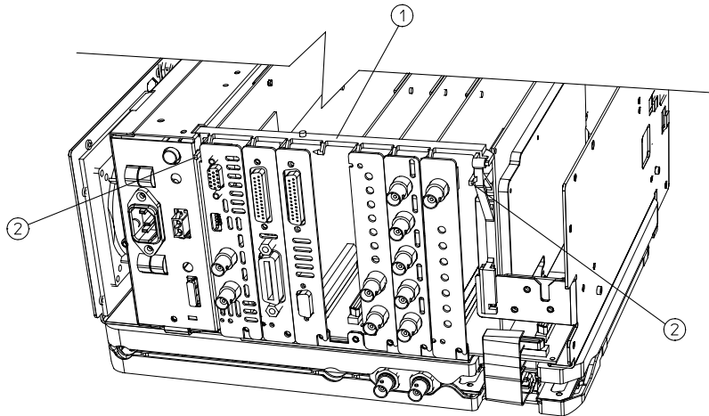
Figure 7 Removing the Vibration Support
